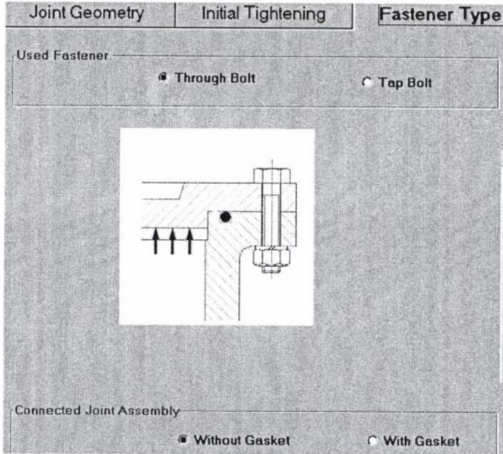
Fig. (4e) : The screen for the Fastener Type .
