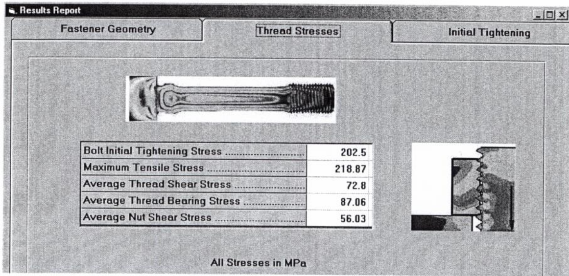
Fig. (4h) : Details of the results on thread stresses .
