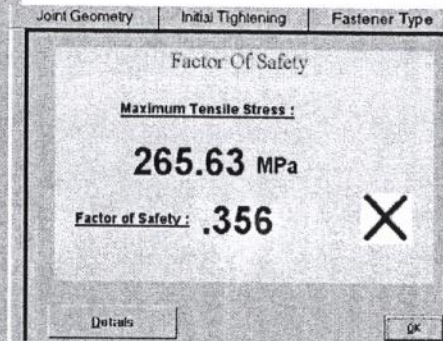
Fig. (4f) : The bolt connection has failed.
